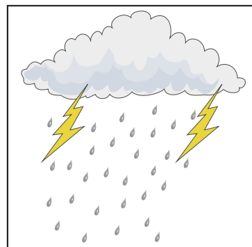
Thunderstorm
