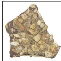
Conglomerate
