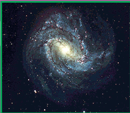
BARRED SPIRAL
