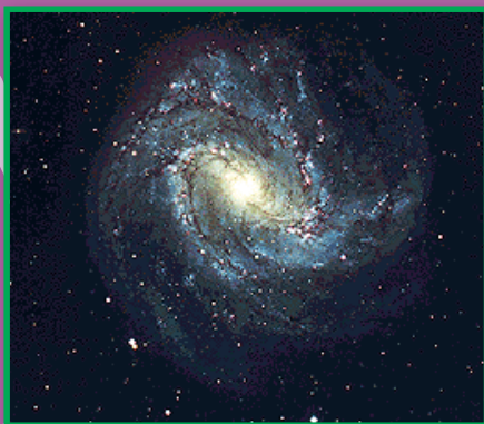
BARRED SPIRAL
