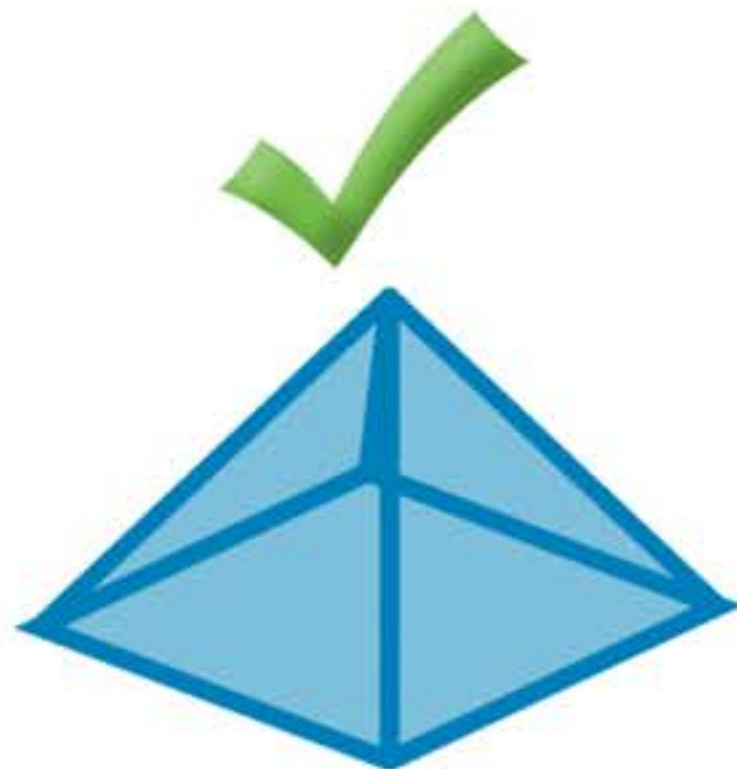
Square Pyramid
