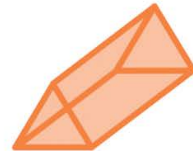
Triangular Prism
